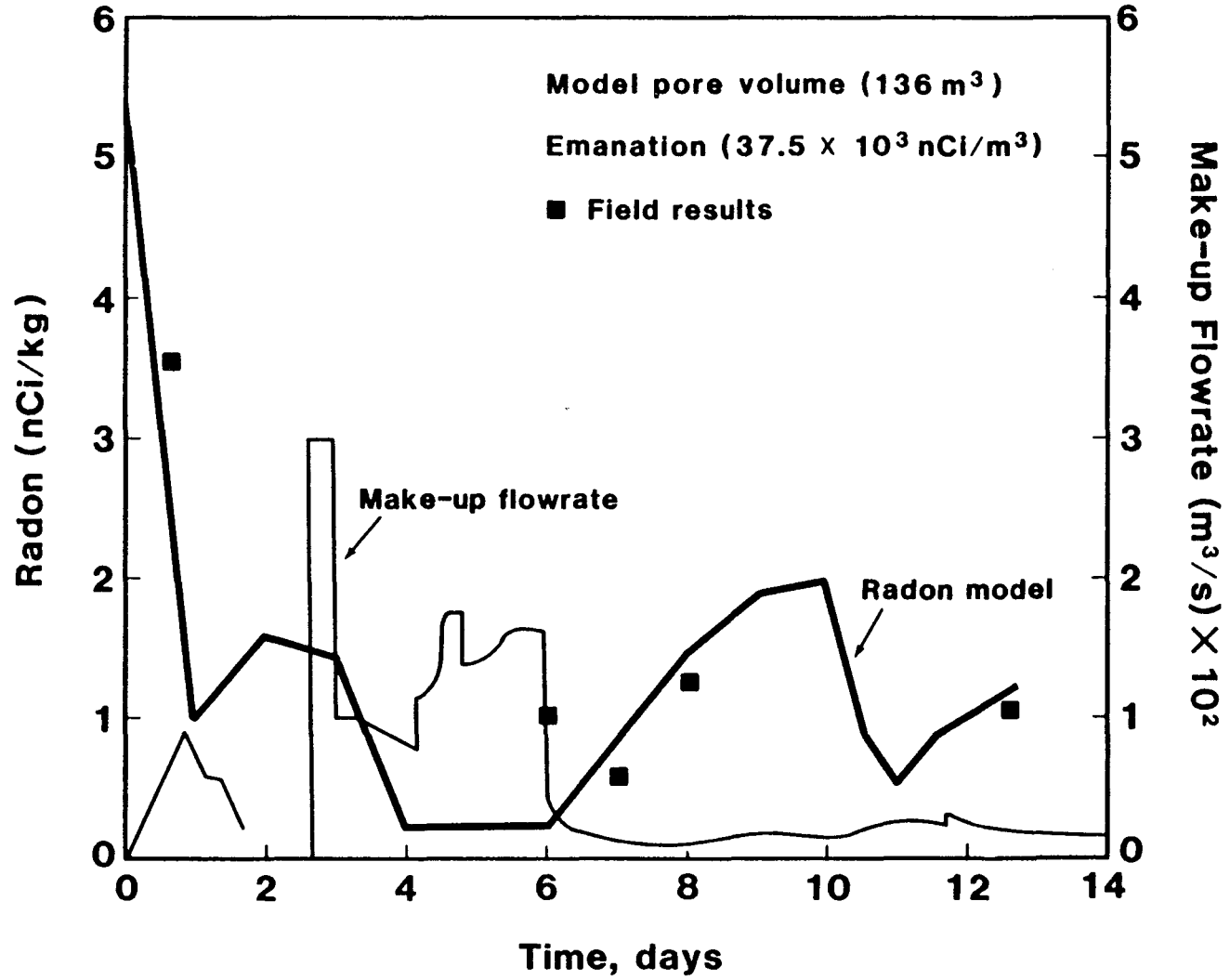
Fig. 2-4: Radon Concentration vs Time Segment 4 Test.
