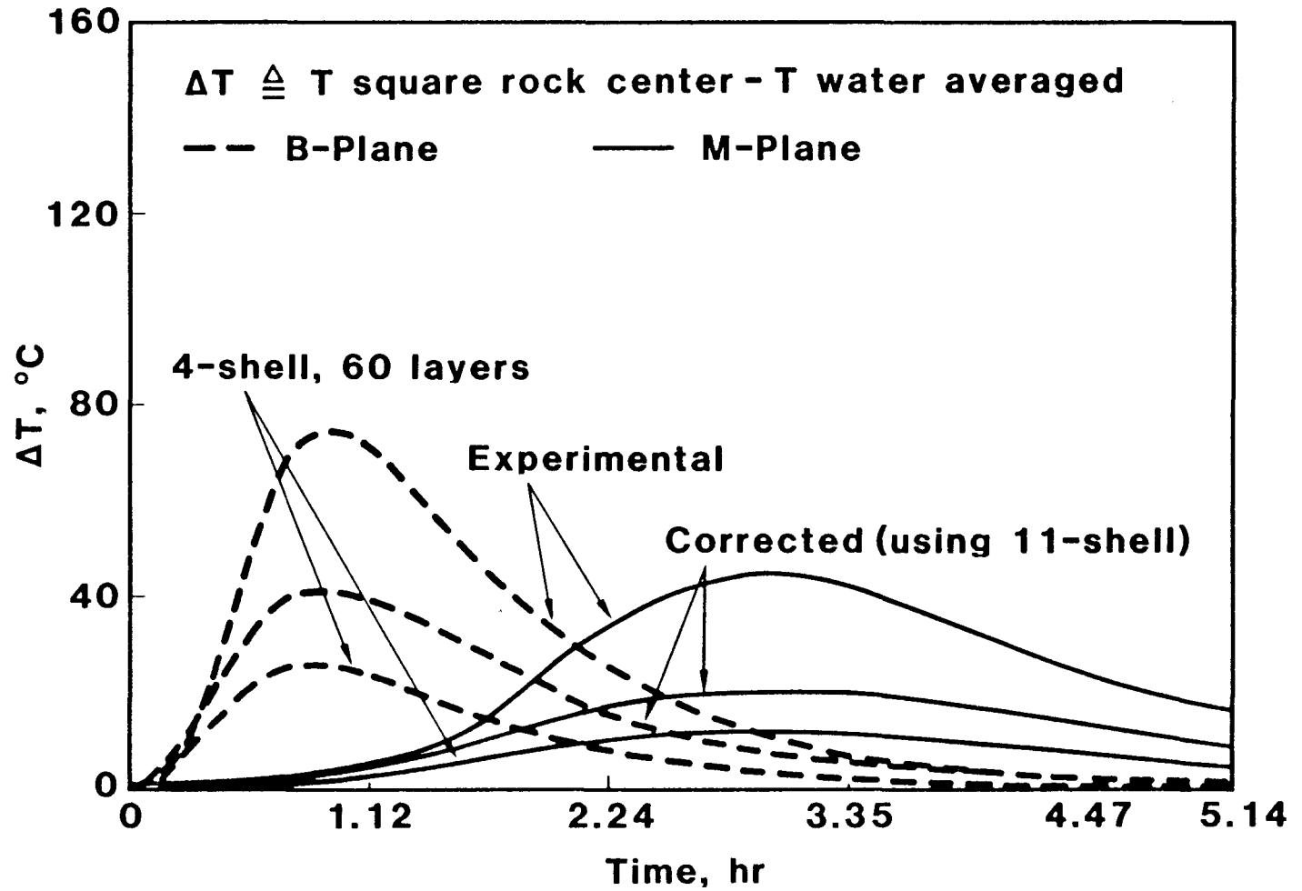
Fig. 1-5: Comparison of Measured and Predicted Rock-Center to Water Temperature Differences for Heat Extraction Experiment Run 5-1.
