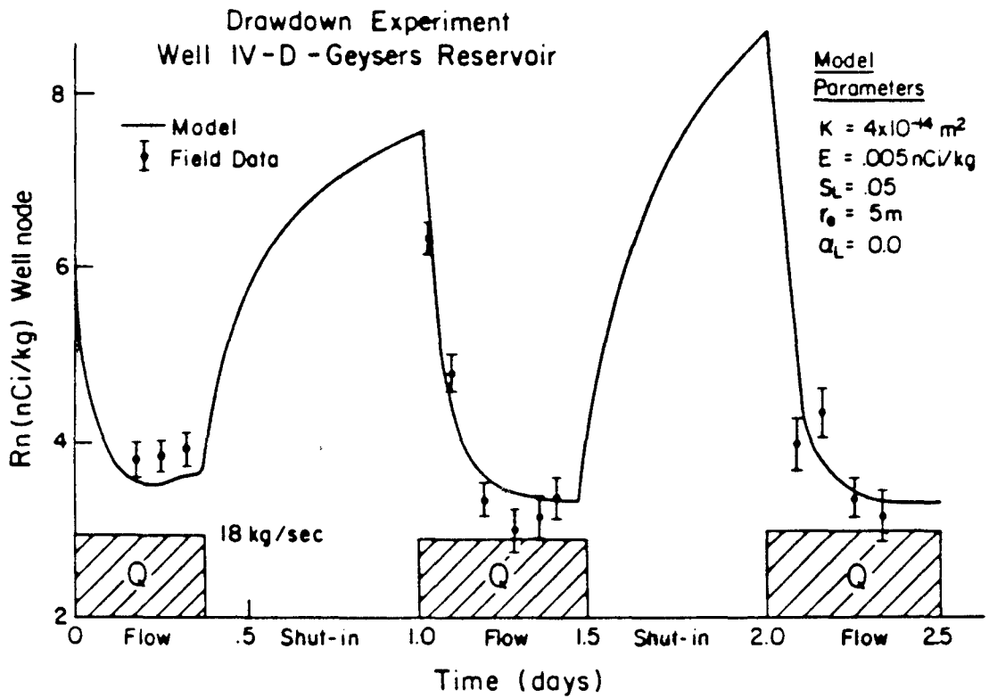
Fig. 2-8: Simulation of Cyclic Drawdown Response at the Geyser.
