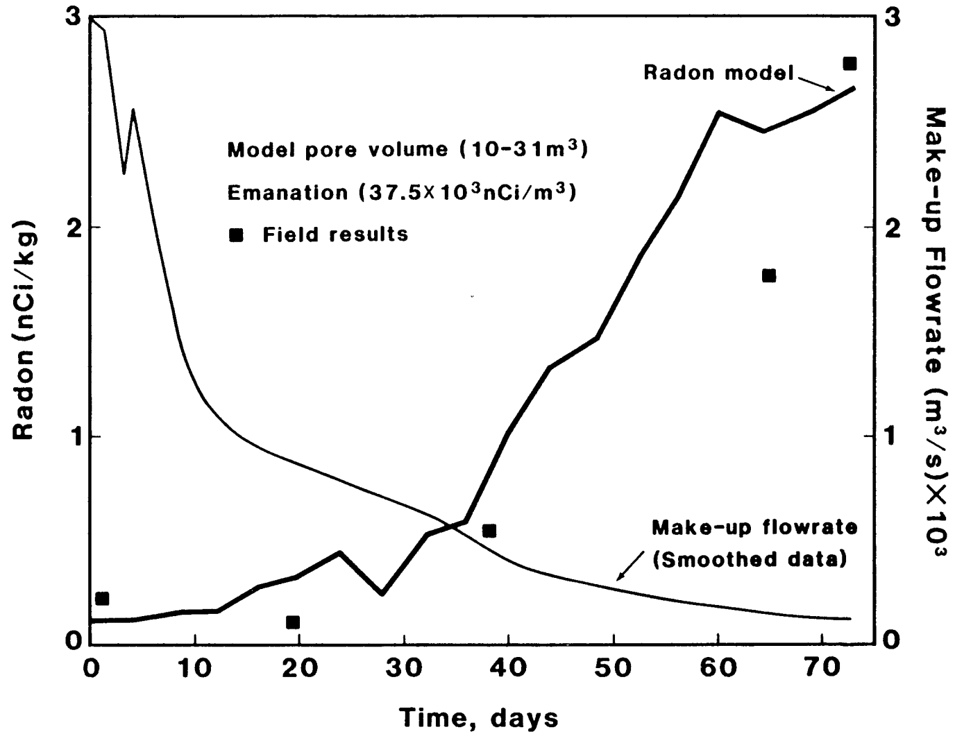
Fig. 2-3: Radon Concentration vs Time Segment 2 Test.
