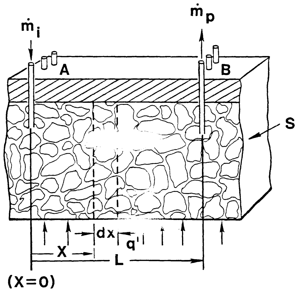
Fig. 1-10: Linear Heat Sweep Model Geometry.
