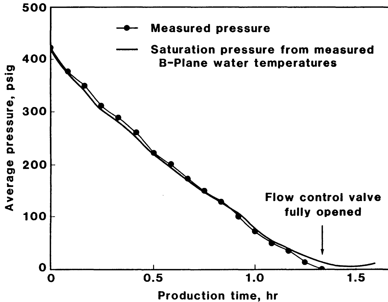
Fig. 1-8: Average Matrix Pressure as a Function of Production Time for Run 5-5.
